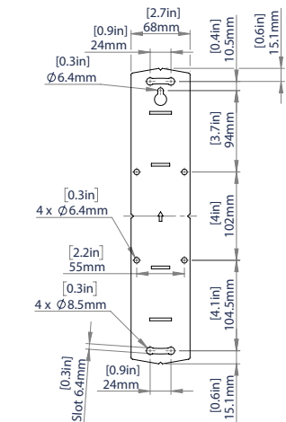
WALL PLATE
